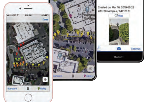
VMap
